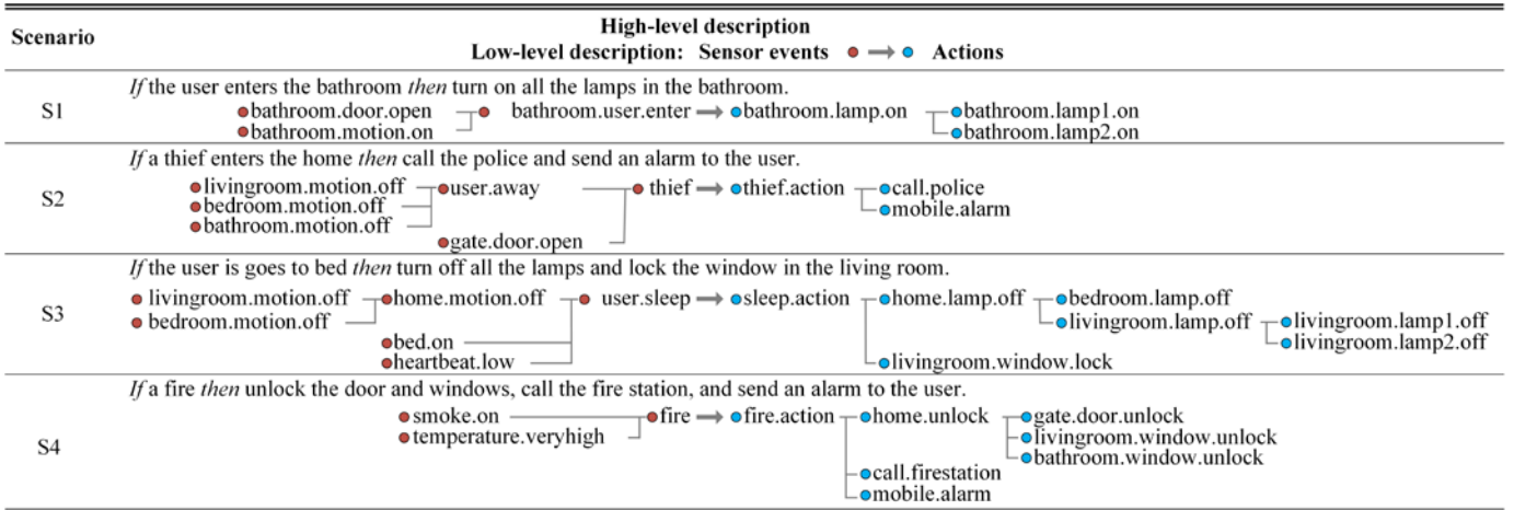
Fig. 6. Four scenarios used in the experiment. S1 is for the training session, and S2, S3, and S4 for the main experiment.
