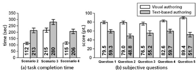
Fig. 9. Average measurements of the user experiment.
