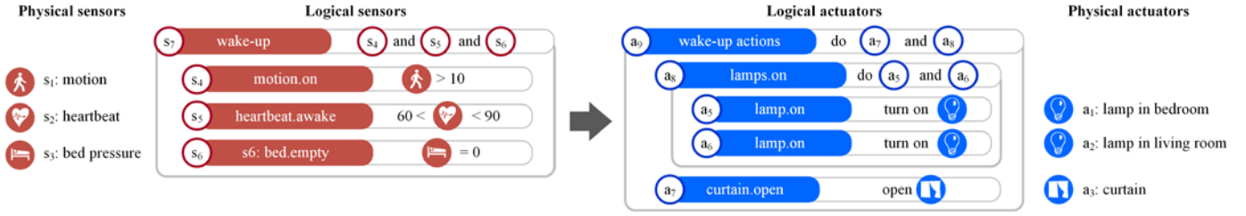
Fig. 1. An example overview of hierarchical abstraction of virtual sensors and actuators. Given the physical sensors and actuators, their hierarchical groupings make logical sensors/actuators. As a result, when the top-level virtual sensor ( s_7 ) detects a user's wake-up event, the top-level virtual actuator ( a_9 ) triggers the actuations of the physical devices.
